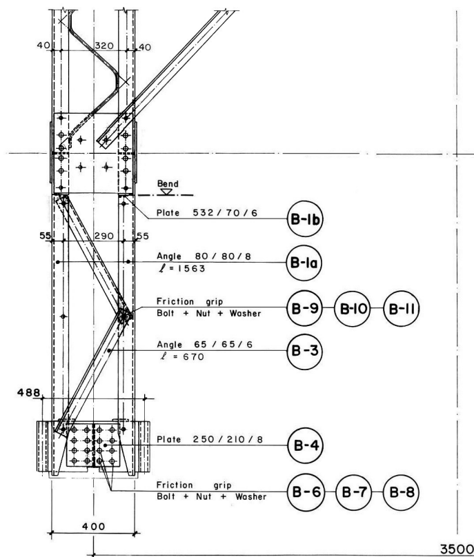
FRONT ELEVATION
