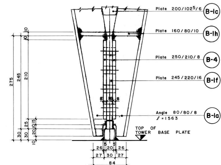
SECTION C-C
