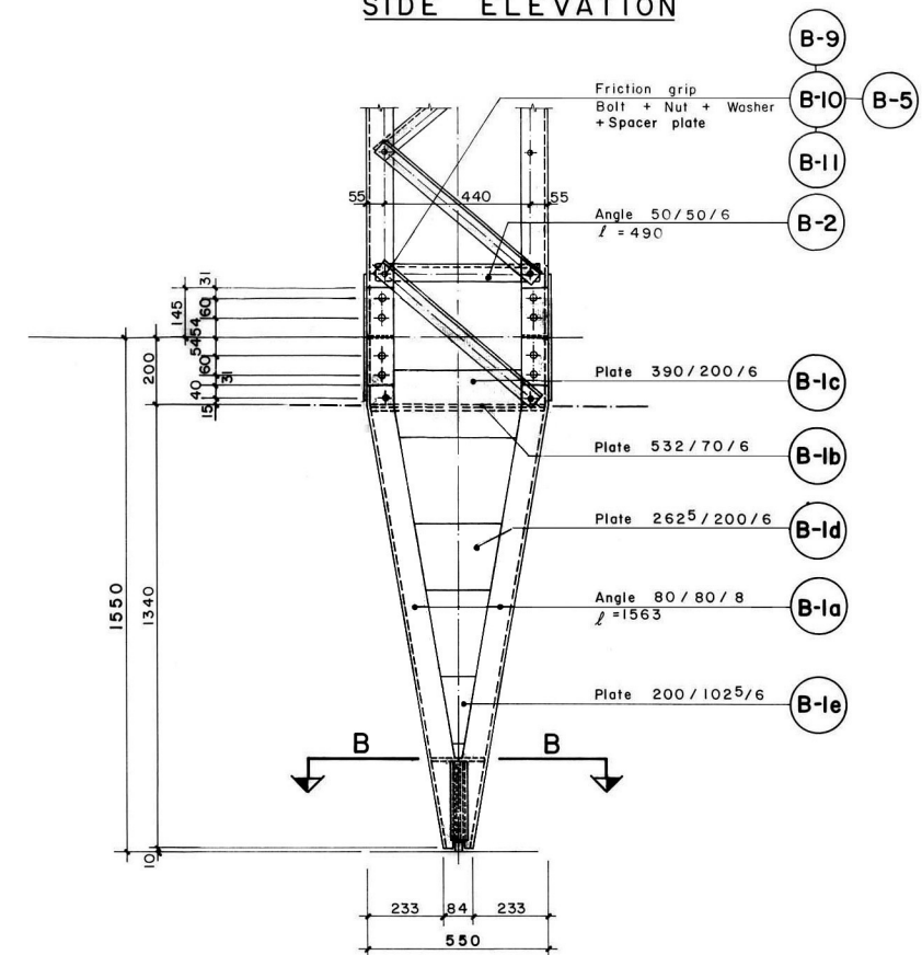
SIDE ELEVATION
