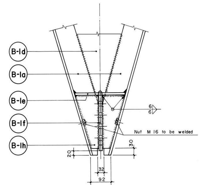
VIEW "B"
