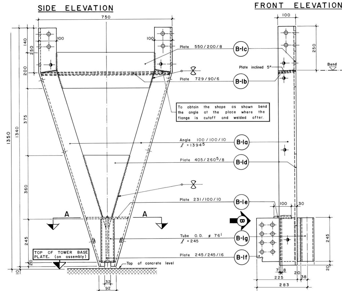
PLAN AT A-A
