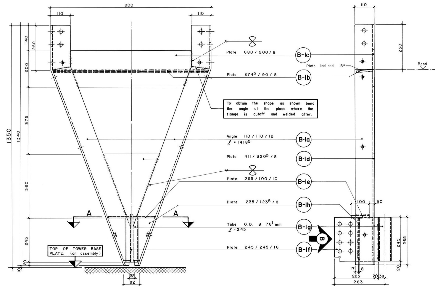
SIDE ELEVATION
