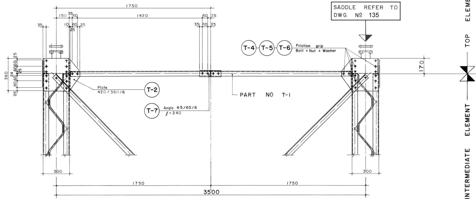
FRONT ELEVATION
