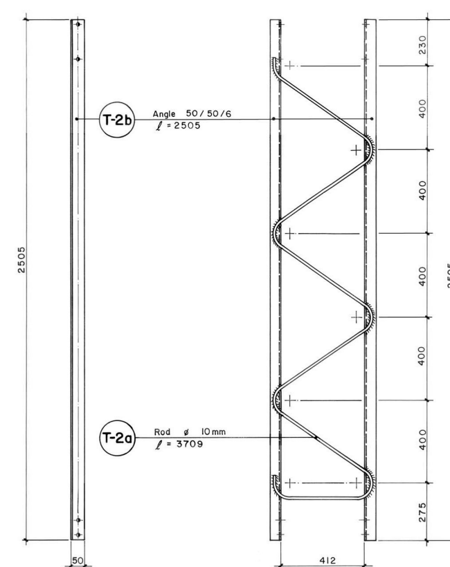
SIDE ELEVATION
