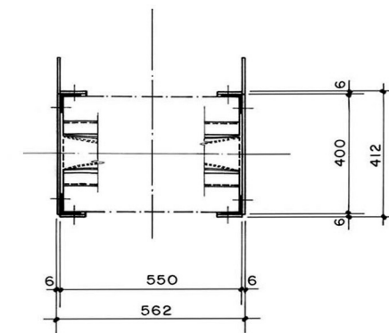
PLAN VIEW A-A
