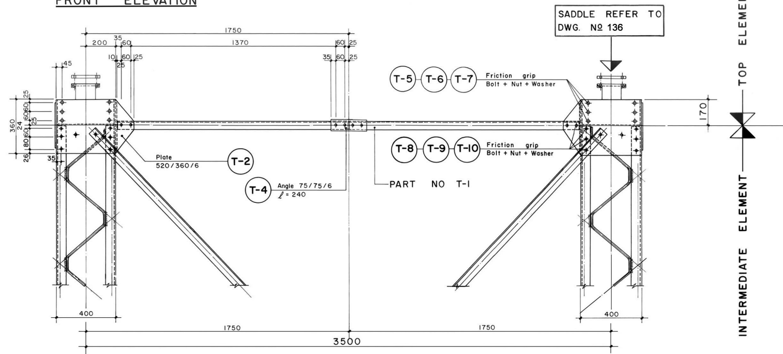
FRONT ELEVATION
