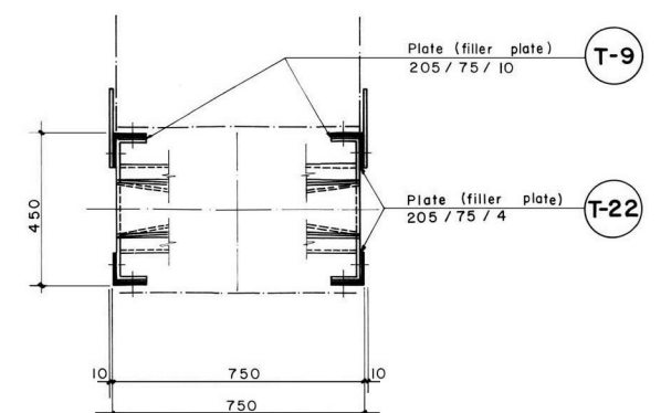
PLAN VIEW A-A
