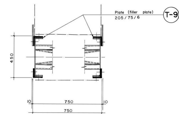
PLAN VIEW A-A
