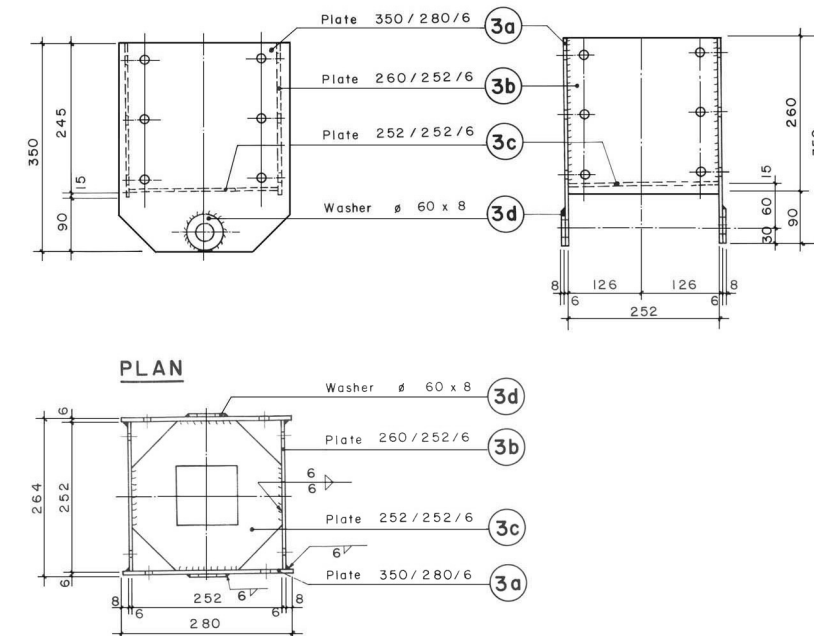
FRONT ELEVATION
