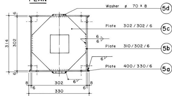
PLAN
