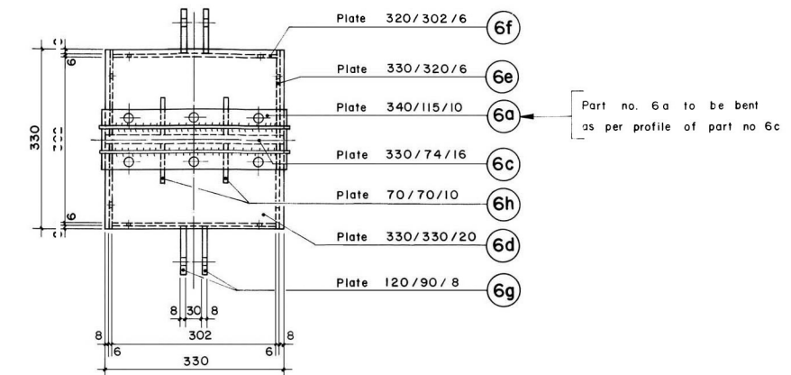
PLAN
