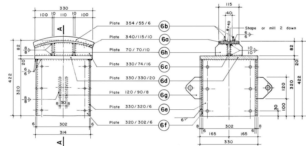
FRONT ELEVATION
