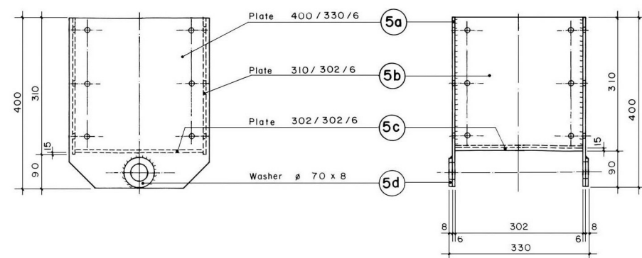
FRONT ELEVATION
