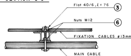
SECTION C-C
