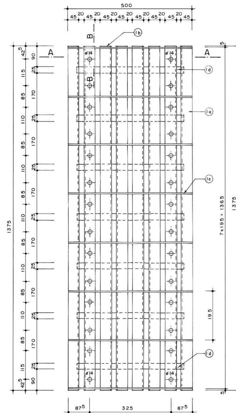
PLAN (SPECIAL PART) (See note 6)
