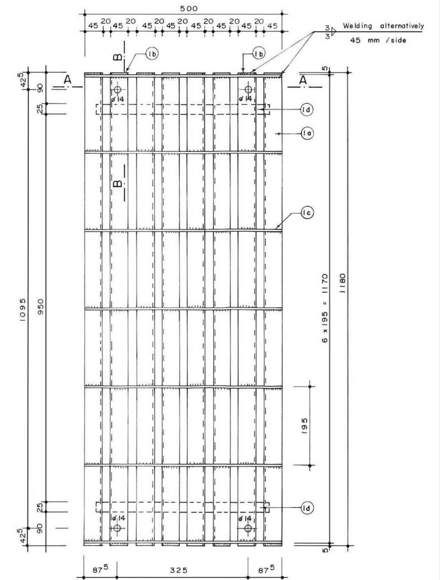
PLAN (STANDARD PART)
