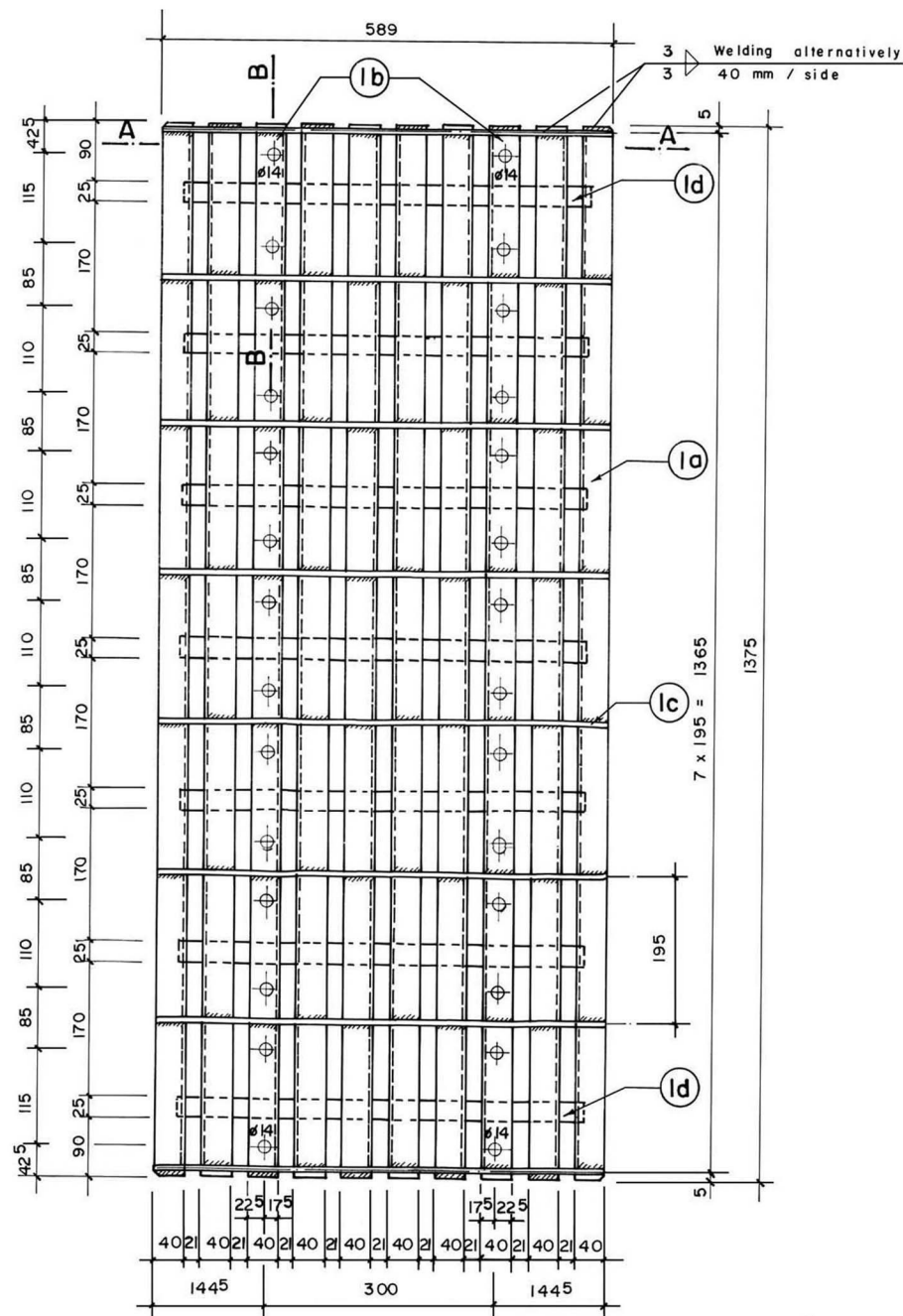
PLAN (SPECIAL PART) (See note 6)
