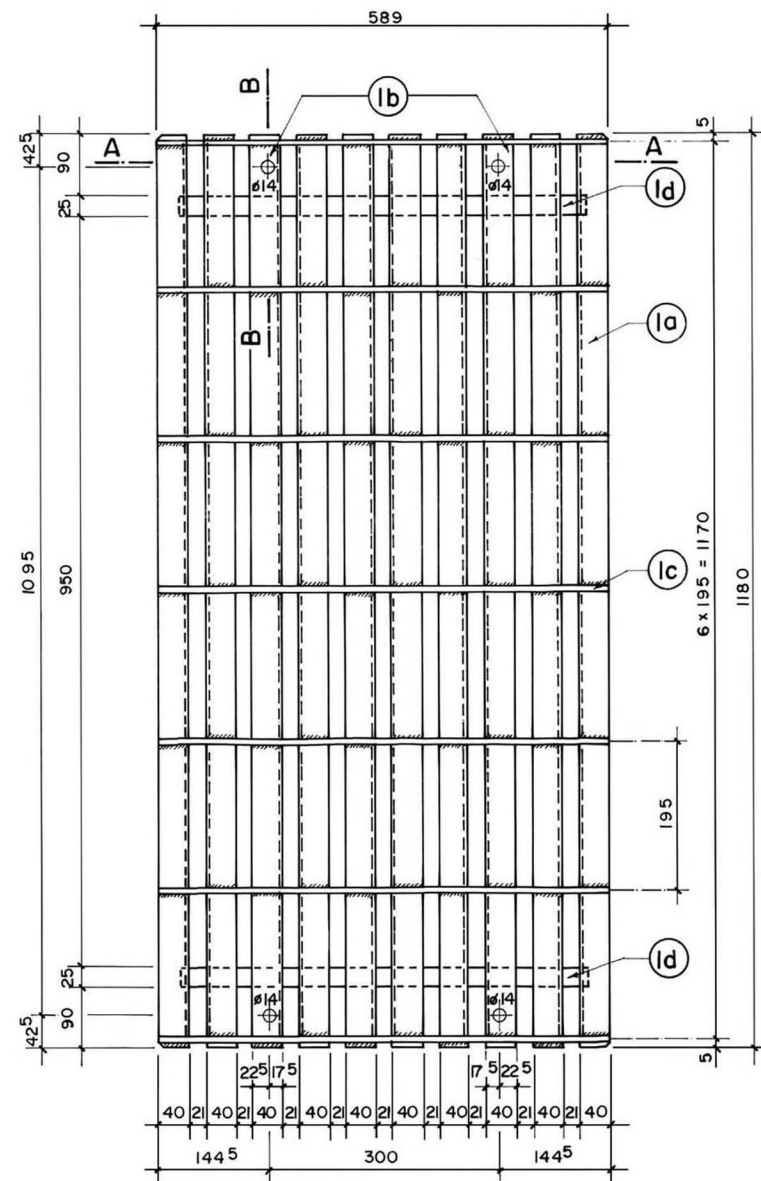
PLAN (STANDARD PART)
