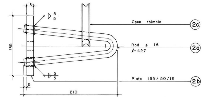
WELDING DETAIL OF PART 2
