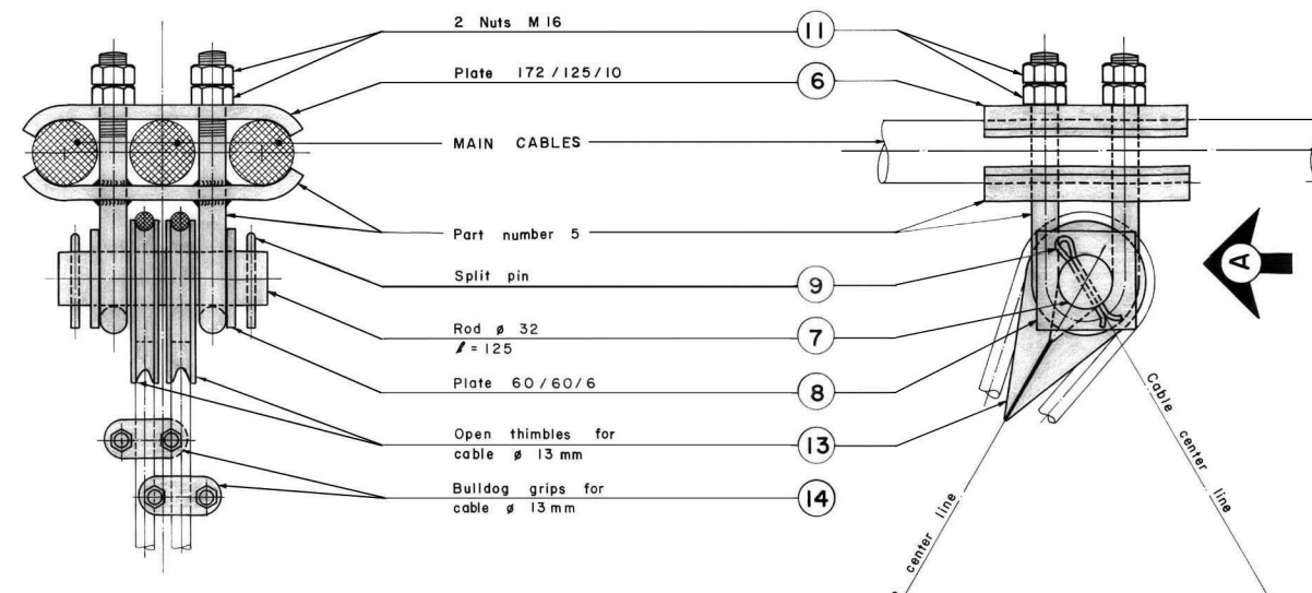
VIEW THROUGH "A"
