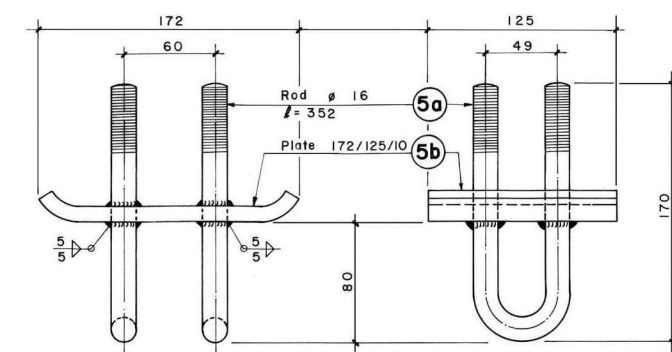
WELDING DETAIL OF PART 5
