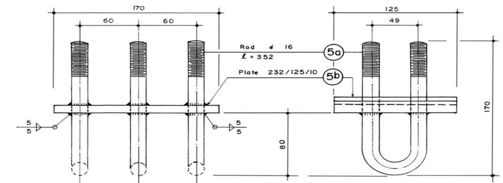
WELDING DETAIL OF PART 5
