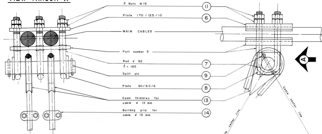
VIEW THROUGH "A"
