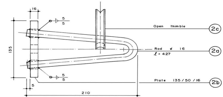
WELDING DETAIL OF PART 2
