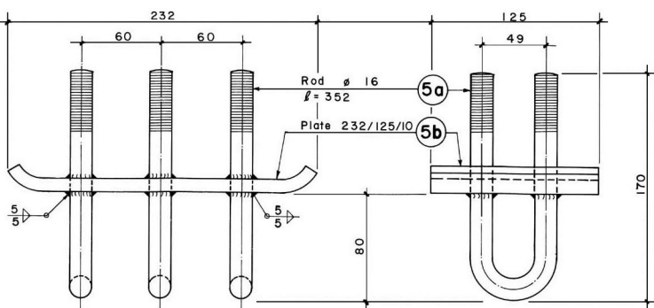
WELDING DETAIL OF PART 5
