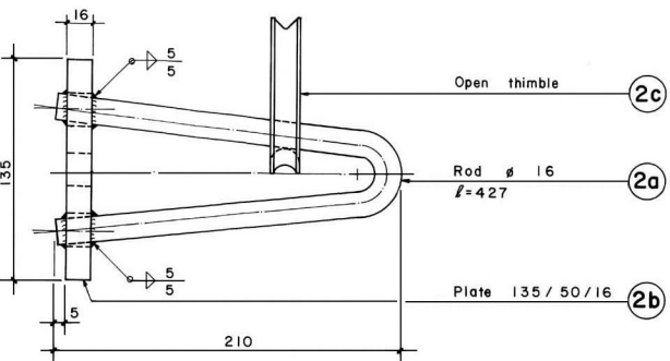
WELDING DETAIL OF PART 2
