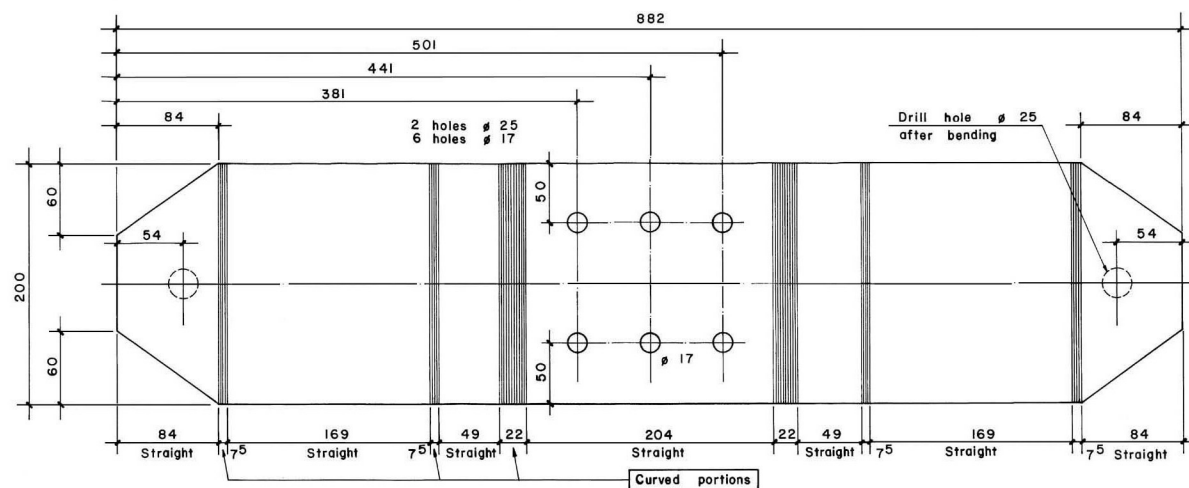
DETAIL OF PART Ia
