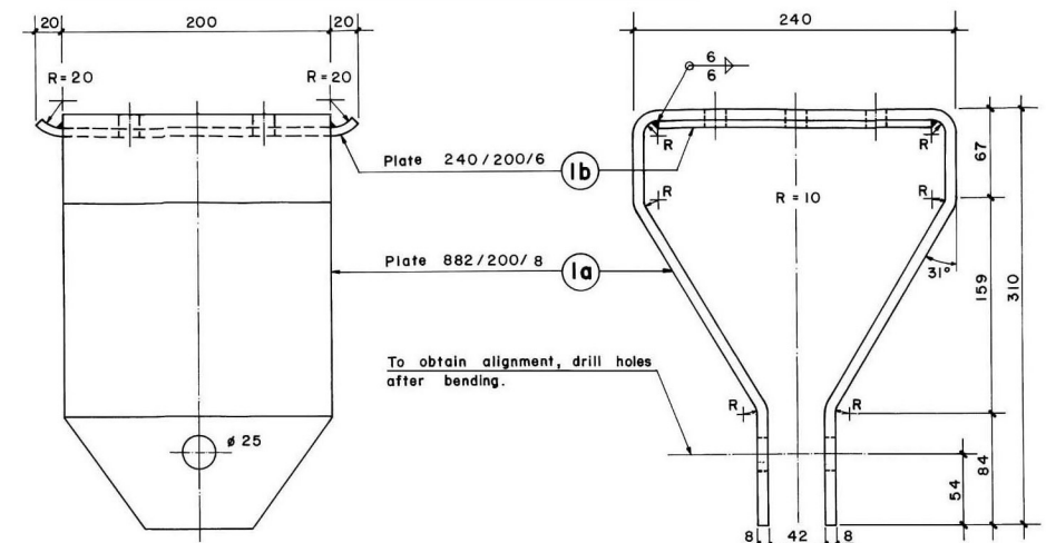
WELDING DETAIL OF PART I
