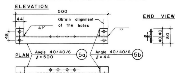
WELDING DETAIL OF PART NO 5
