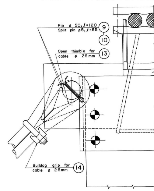
CONNECTION DETAIL AT TOWER
