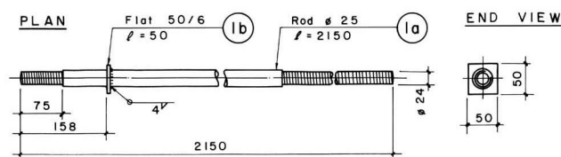
WELDING DETAIL OF PART NO 1
