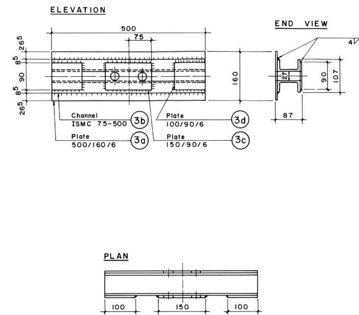
WELDING DETAIL OF PART NO 3
